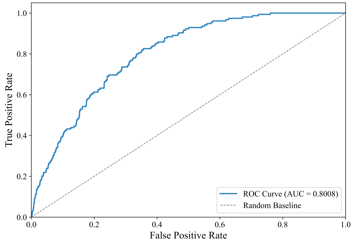
ROC Curve — SWEDISH_MANUAL (intfloat/multilingual-e5-large-instruct, Random_Forest)
