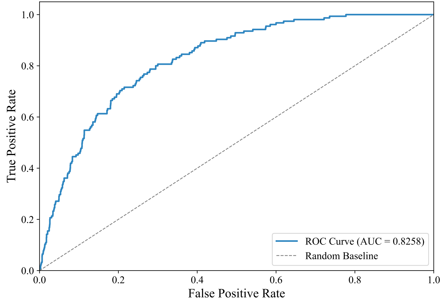
ROC Curve — SWEDISH_MANUAL (intfloat/multilingual-e5-large-instruct, Voting_Ensemble)
