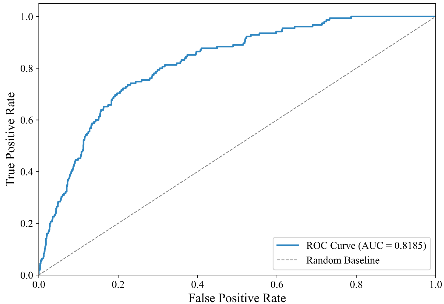
ROC Curve — SWEDISH_MANUAL (intfloat/multilingual-e5-large-instruct, XGBoost)
