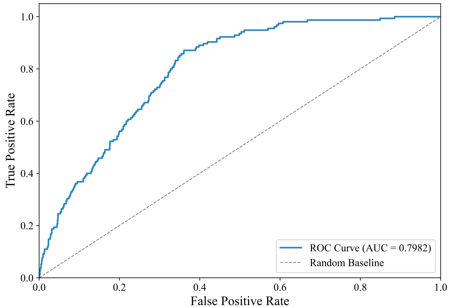
ROC Curve — SWEDISH_MANUAL (upskyy/bge-m3-korean, Random_Forest)
