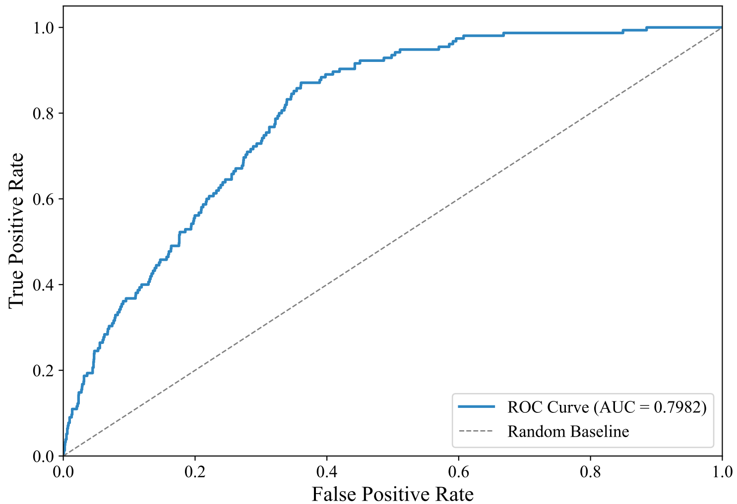
ROC Curve — SWEDISH_MANUAL (upskyy/bge-m3-korean, Random_Forest_Optimized)
