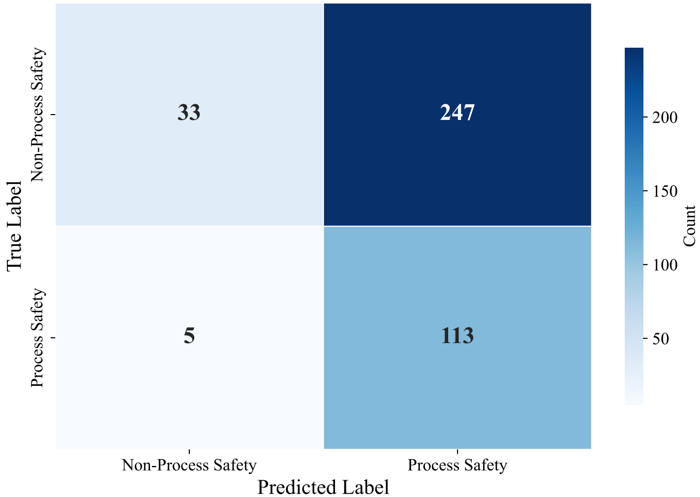
Confusion Matrix — DUTCH_MANUAL (bert-base-multilingual-uncased, svm_linear)
