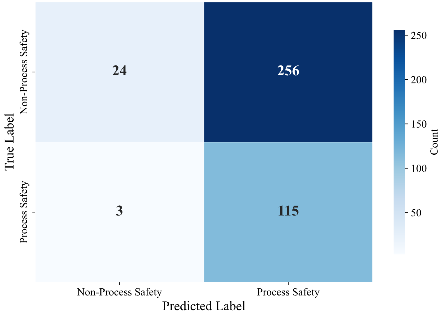
Confusion Matrix — DUTCH_MANUAL (bert-base-multilingual-uncased, xgboost)
