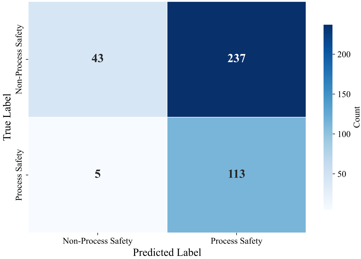
Confusion Matrix — DUTCH_MANUAL (multilingual-e5-large-instruct, lightgbm)
