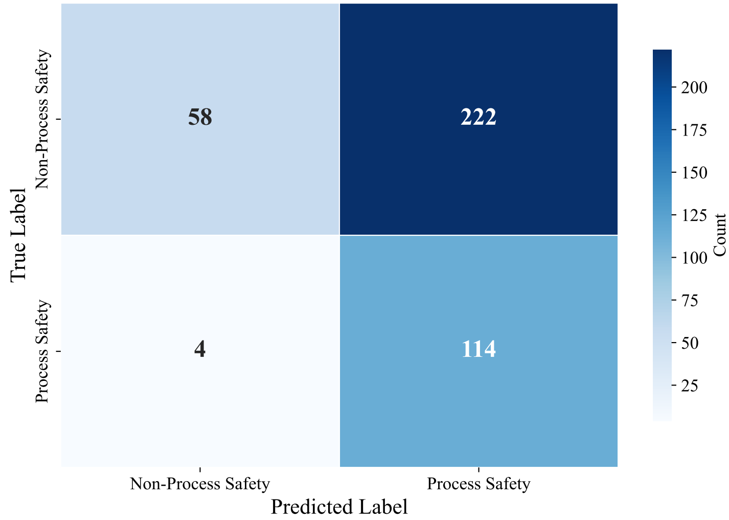
Confusion Matrix — DUTCH_MANUAL (paraphrase-multilingual-MiniLM-L12-v2, svm_rbf)
