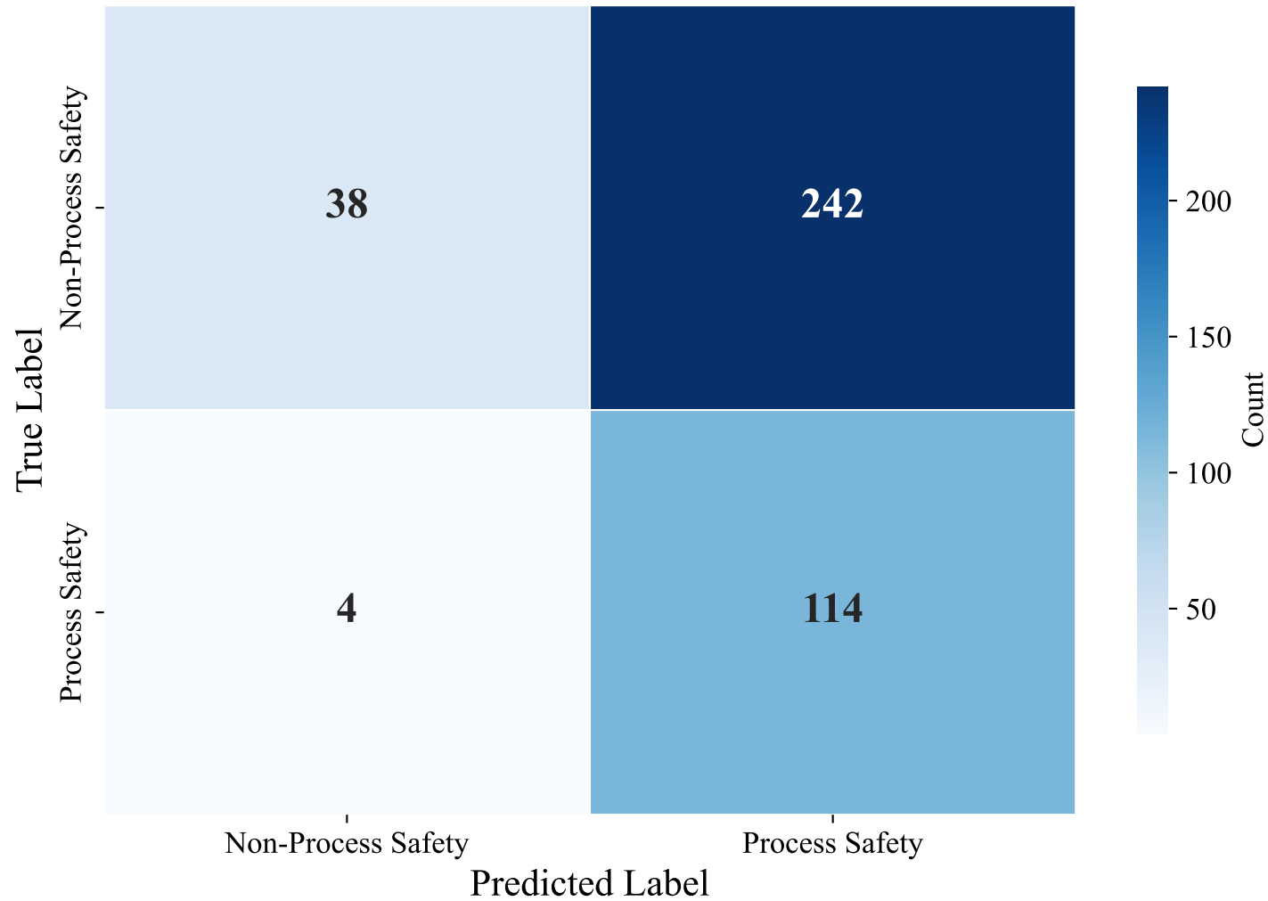
Confusion Matrix — DUTCH_MANUAL (paraphrase-multilingual-mpnet-base-v2, svm_linear)
