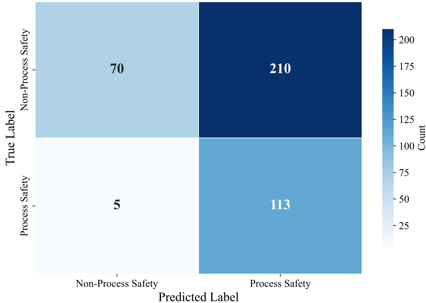
Confusion Matrix — DUTCH_MANUAL (paraphrase-multilingual-mpnet-base-v2, svm_rbf)
