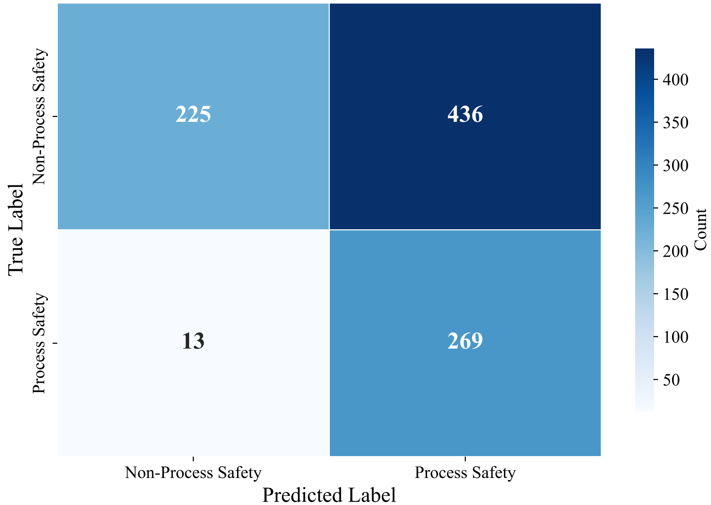
Confusion Matrix — ENGLISH_MANUAL (multilingual-e5-large-instruct, svm_rbf)
