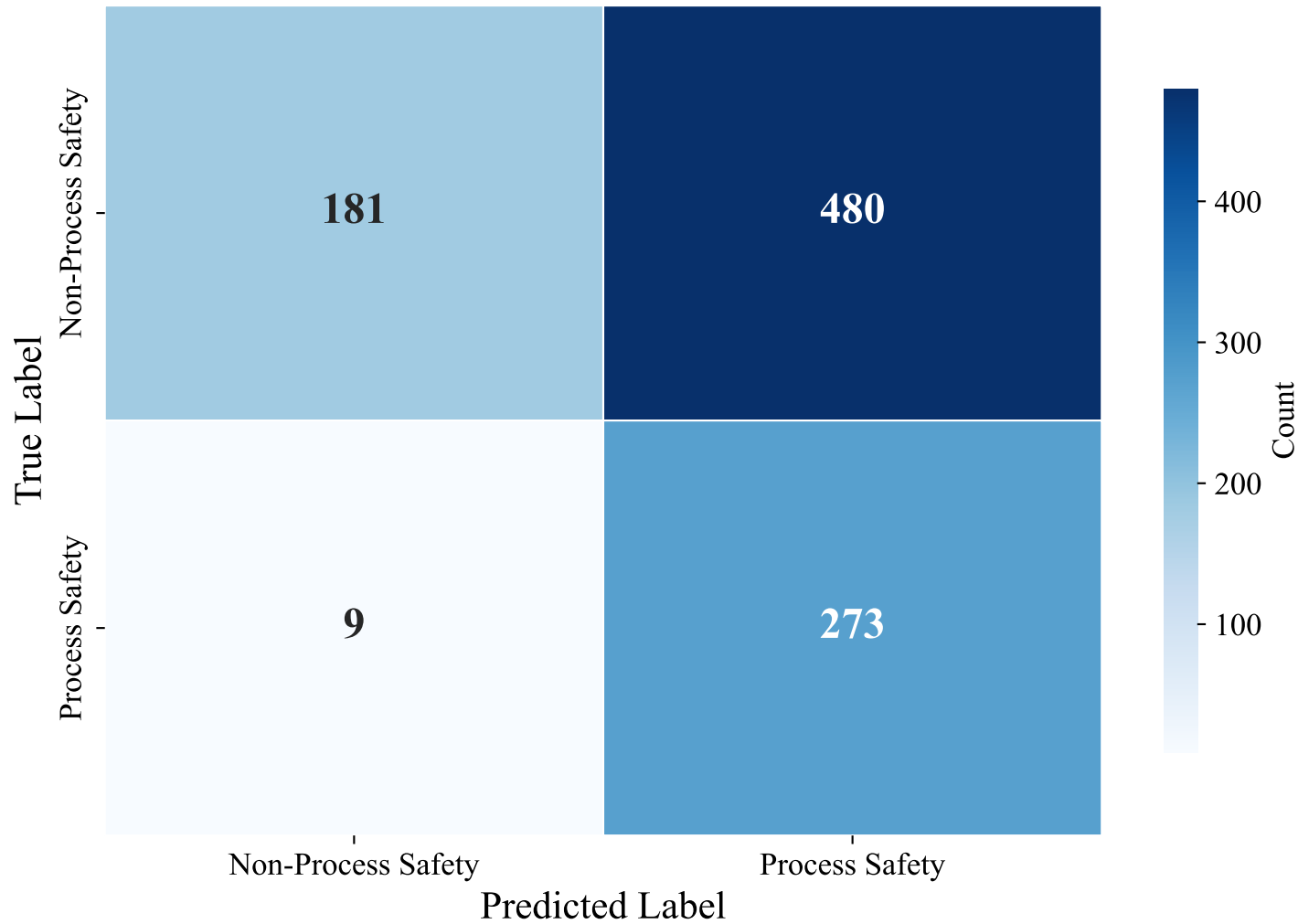
Confusion Matrix — ENGLISH_MANUAL (paraphrase-multilingual-MiniLM-L12-v2, svm_rbf)
