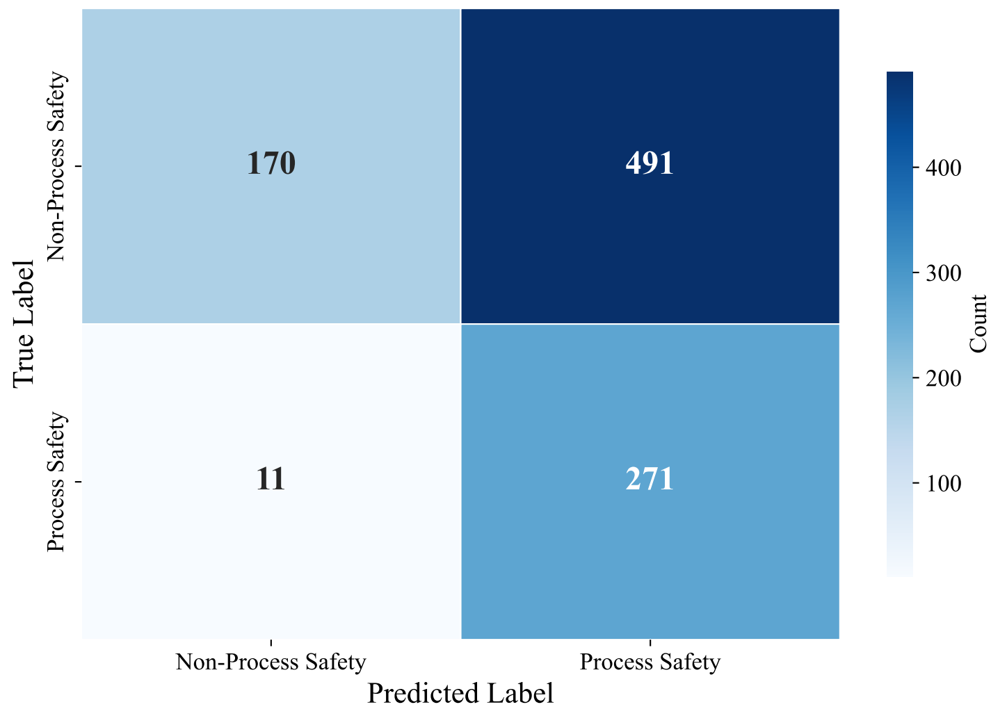
Confusion Matrix — ENGLISH_MANUAL (paraphrase-multilingual-mpnet-base-v2, lightgbm)
