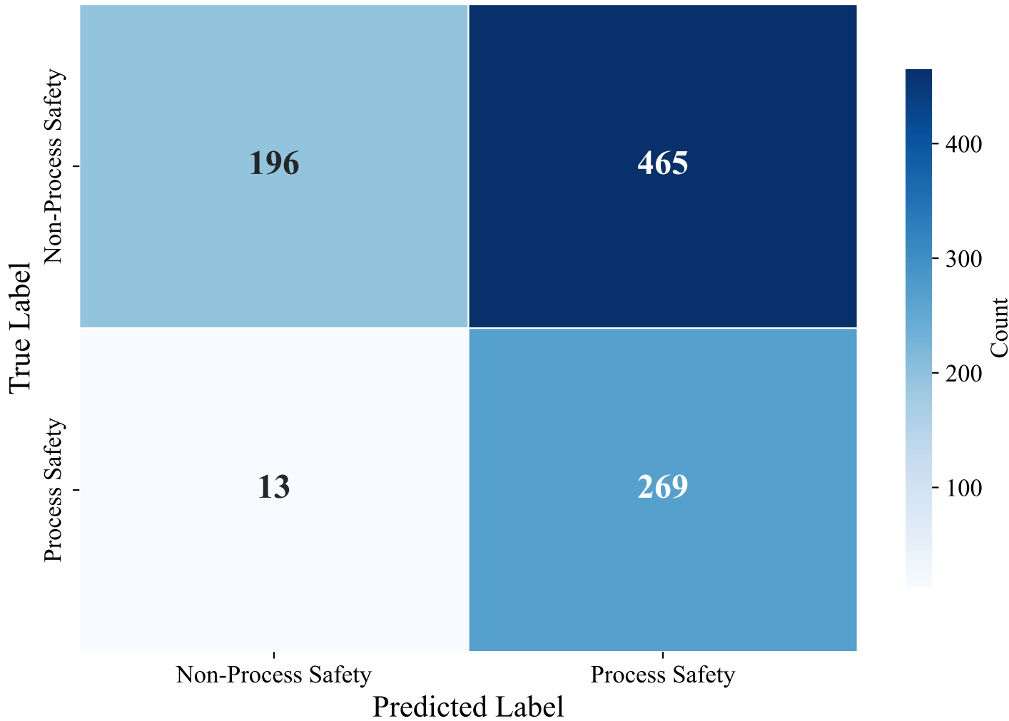
Confusion Matrix — ENGLISH_MANUAL (paraphrase-multilingual-mpnet-base-v2, svm_linear)
