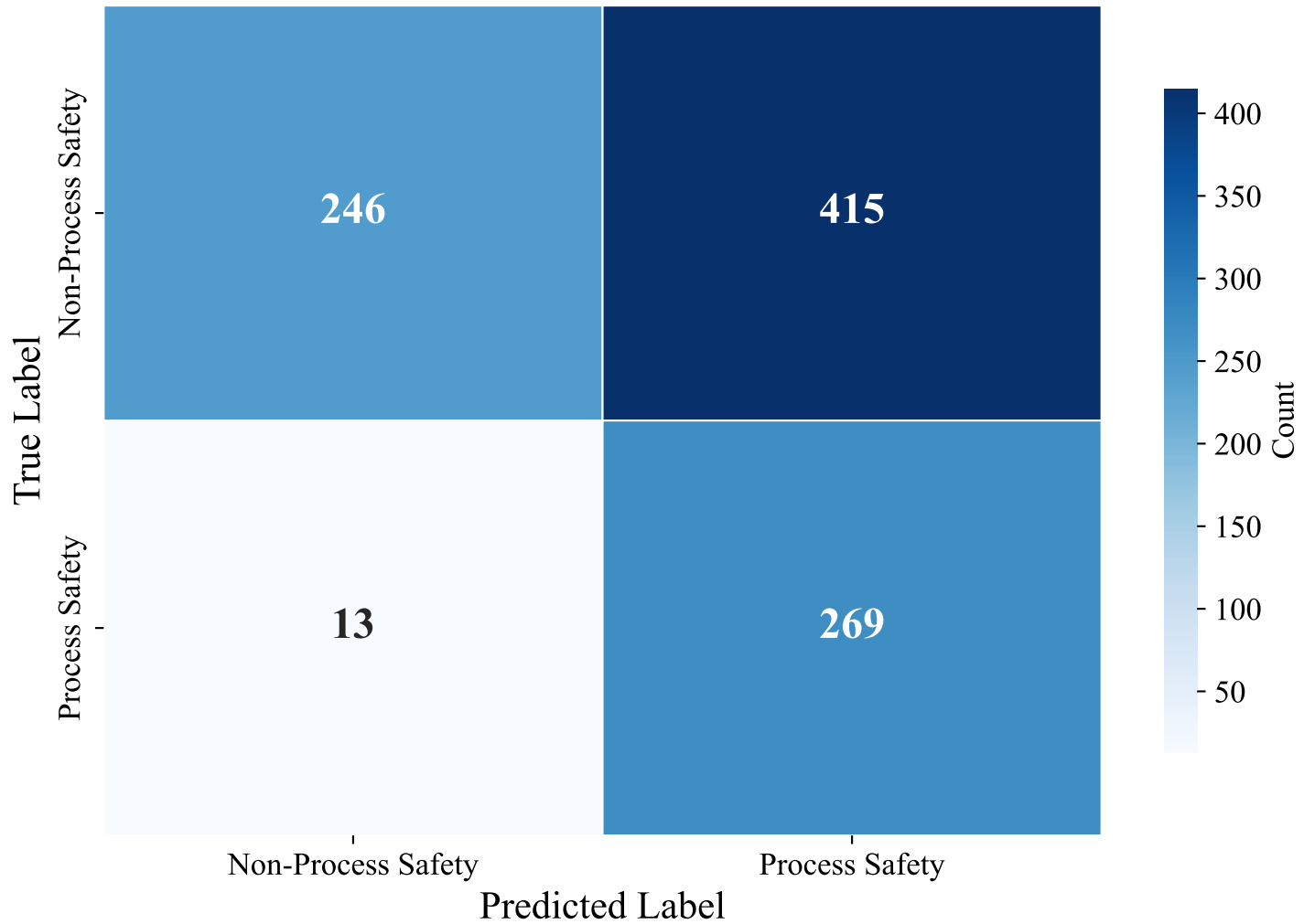
Confusion Matrix — ENGLISH_MANUAL (paraphrase-multilingual-mpnet-base-v2, svm_rbf)
