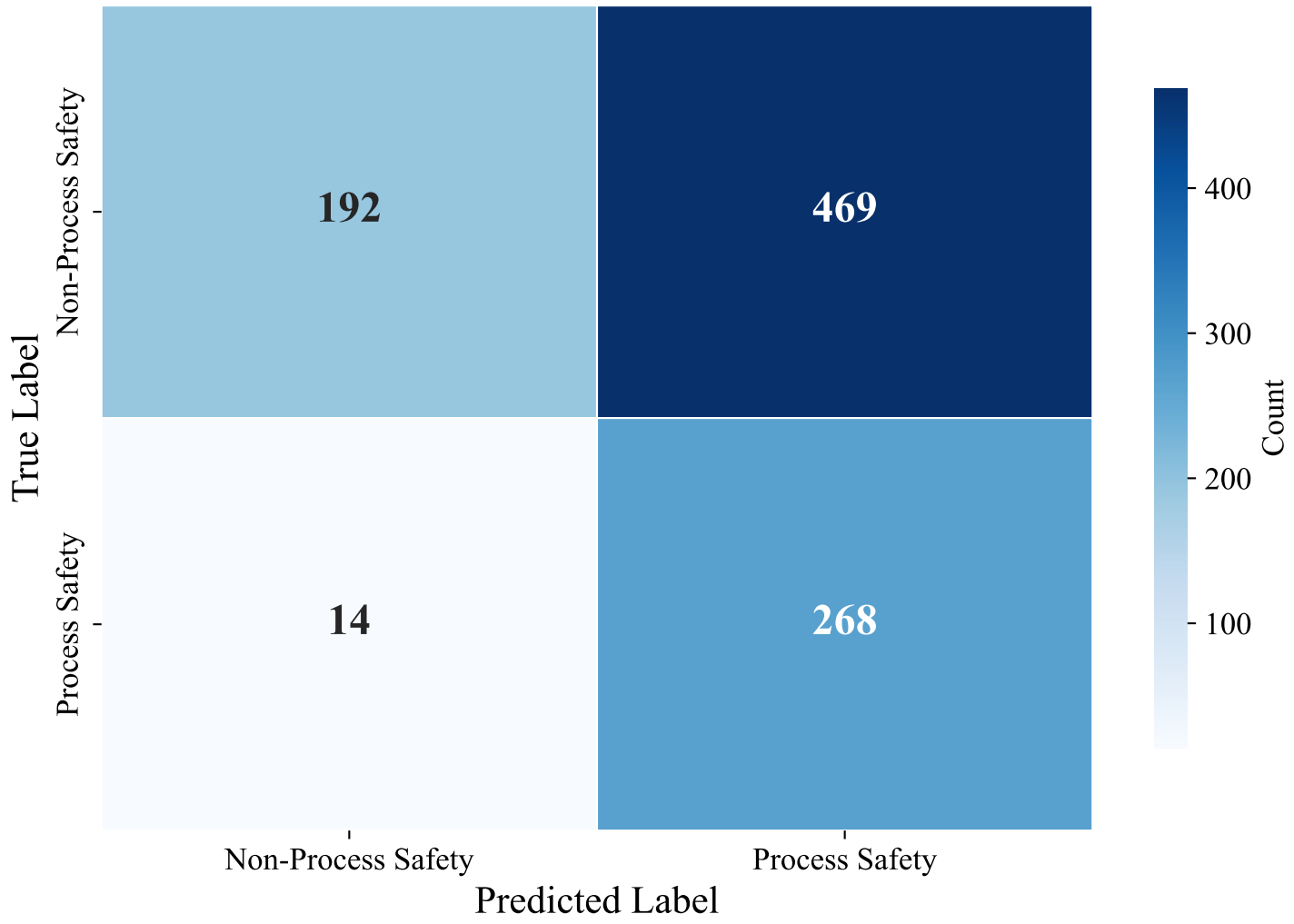
Confusion Matrix — ENGLISH_MANUAL (xlm-roberta-base, svm_linear)
