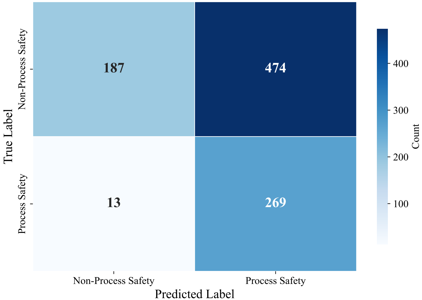
Confusion Matrix — ENGLISH_MANUAL (xlm-roberta-base, svm_rbf)
