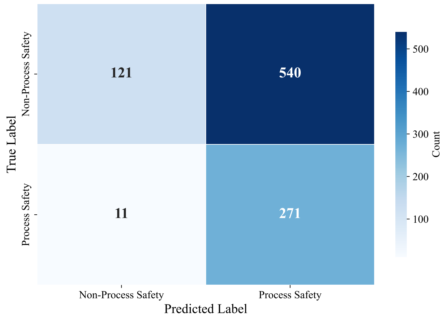
Confusion Matrix — ENGLISH_MANUAL (xlm-roberta-base, xgboost)
