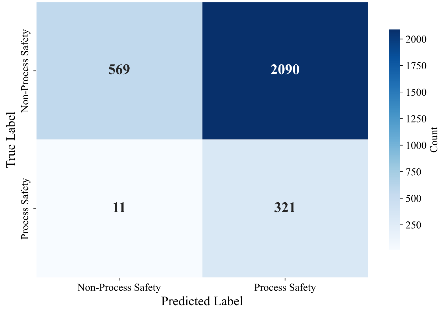
Confusion Matrix — GERMAN_MANUAL (bert-base-multilingual-uncased, svm_linear)
