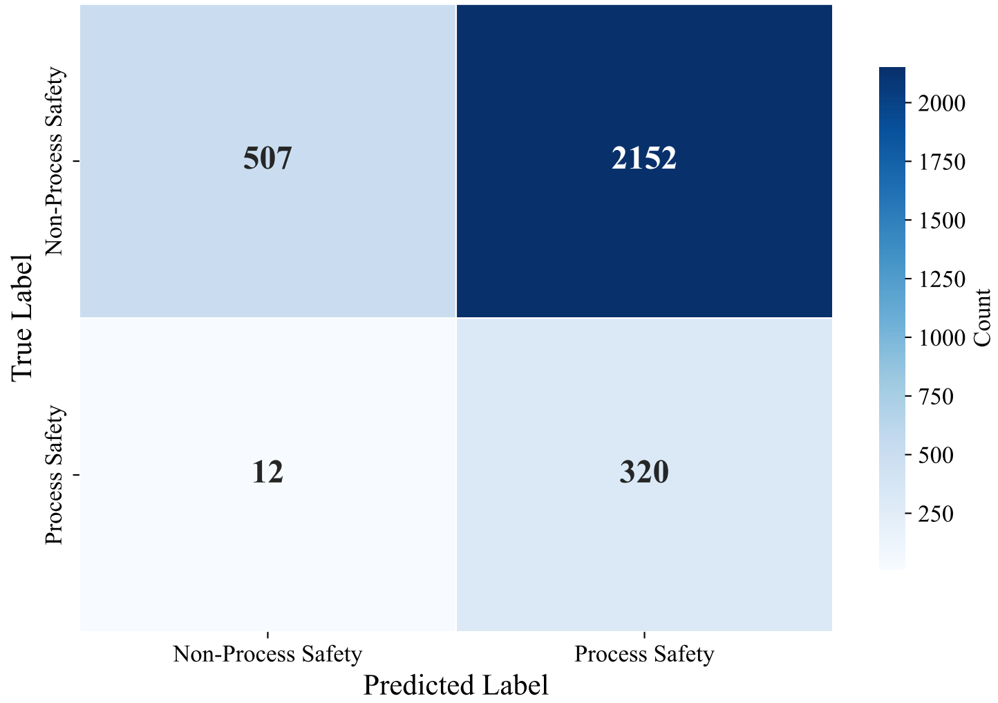
Confusion Matrix — GERMAN_MANUAL (multilingual-e5-large-instruct, random_forest)
