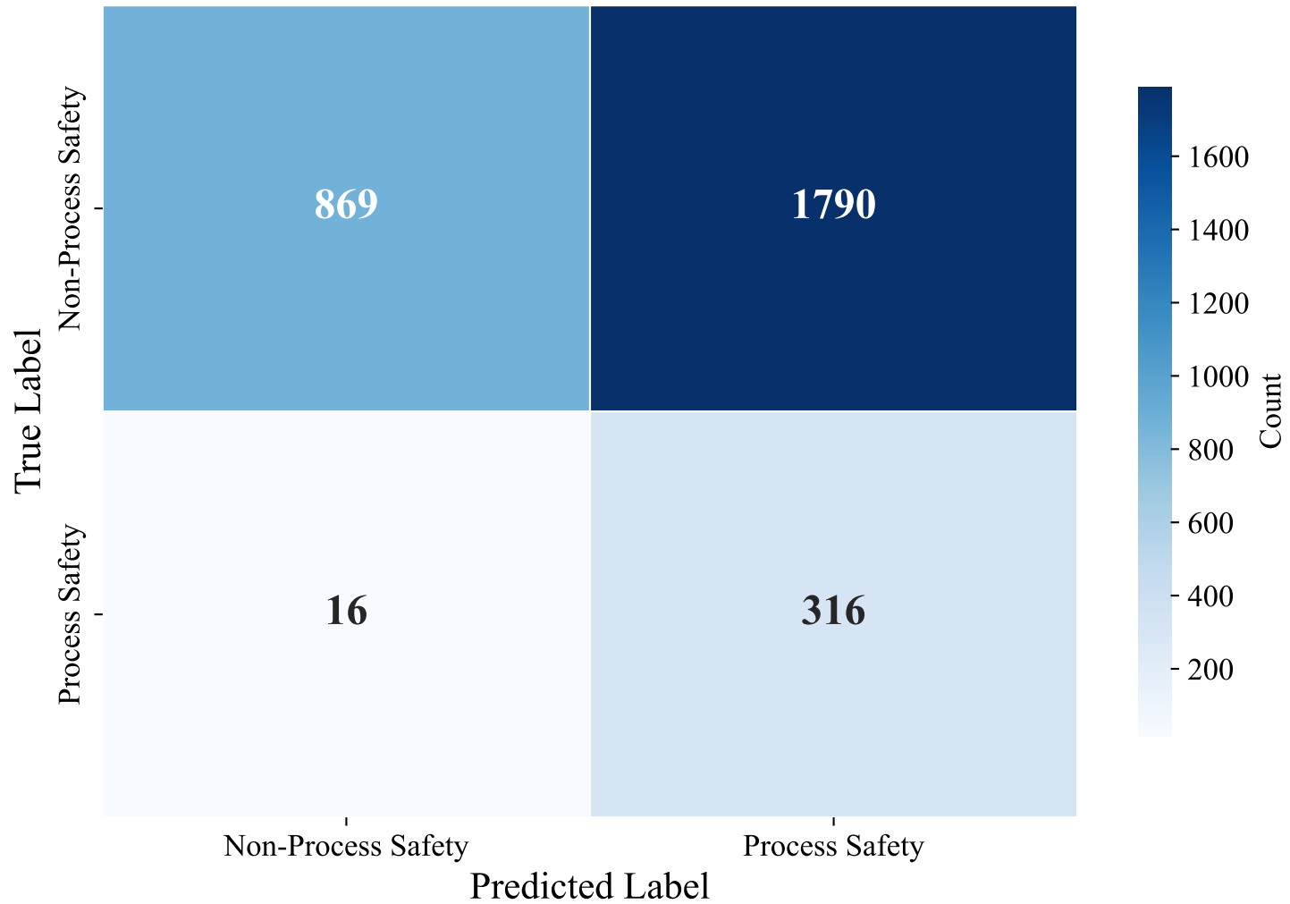
Confusion Matrix — GERMAN_MANUAL (multilingual-e5-large-instruct, svm_rbf)
