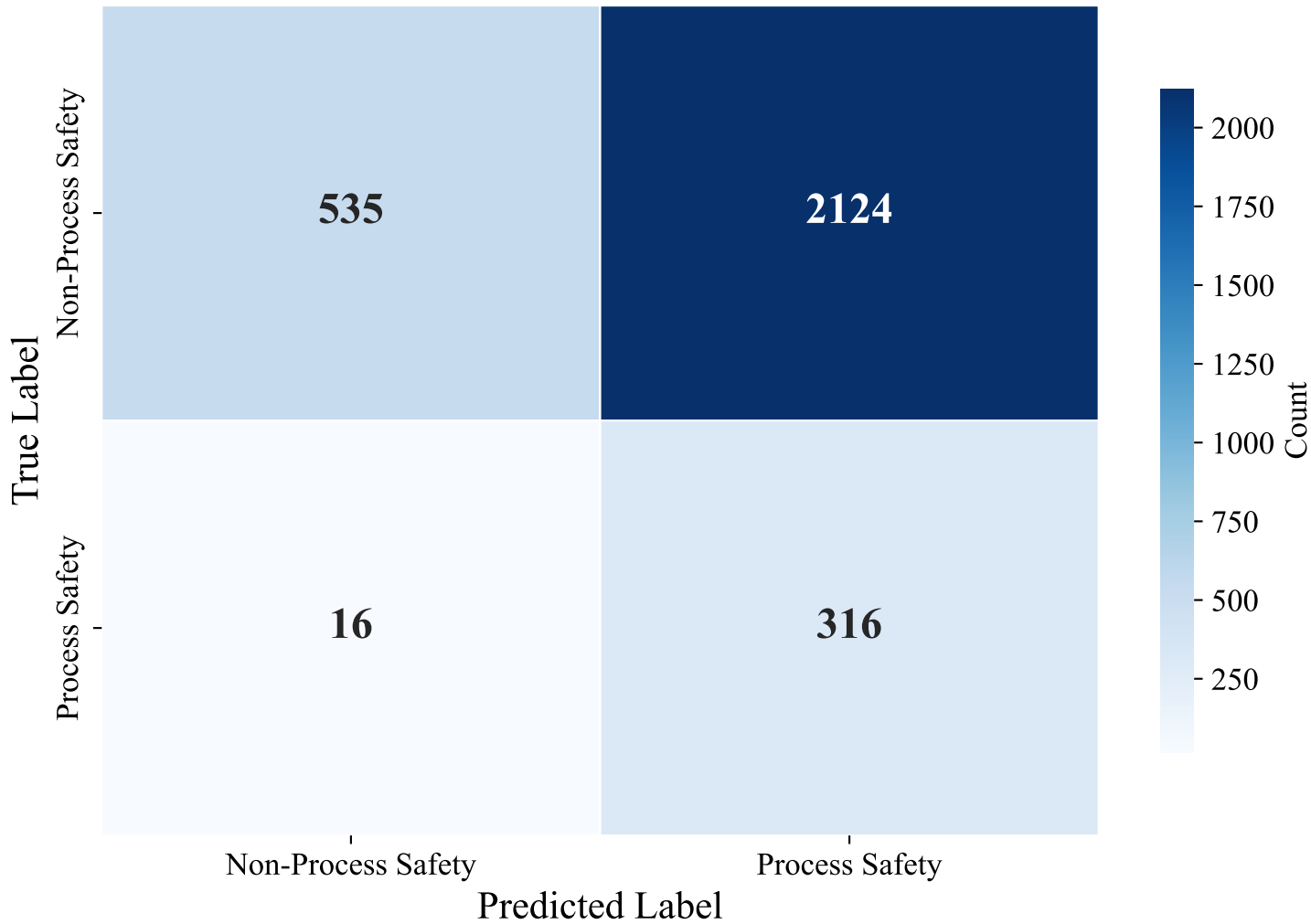
Confusion Matrix — GERMAN_MANUAL (paraphrase-multilingual-mpnet-base-v2, svm_linear)
