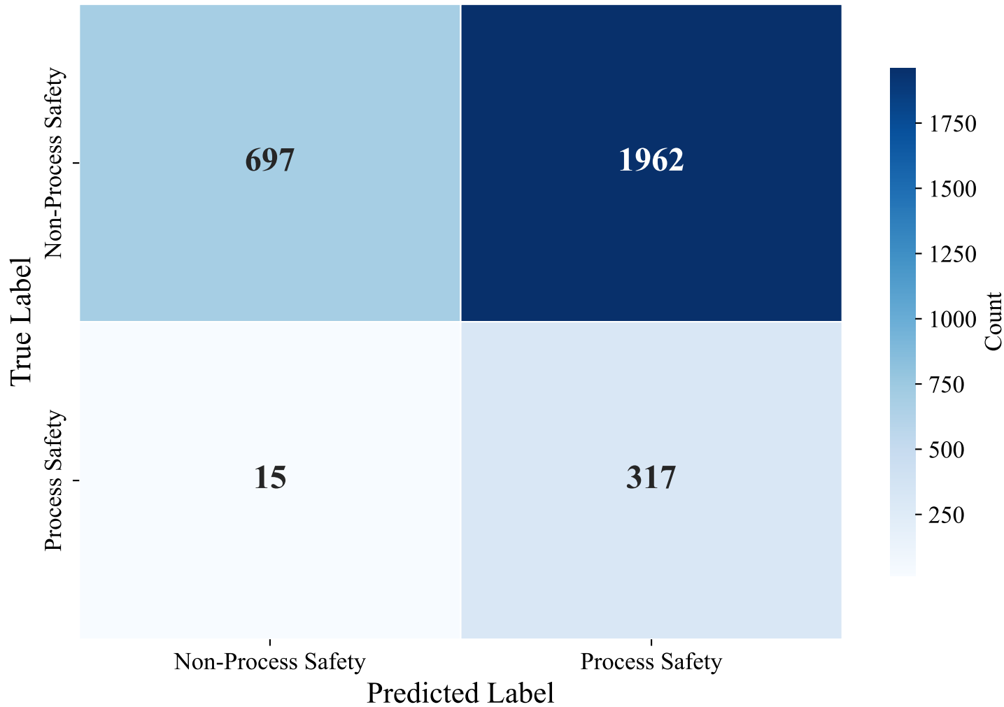
Confusion Matrix — GERMAN_MANUAL (paraphrase-multilingual-mpnet-base-v2, svm_rbf)
