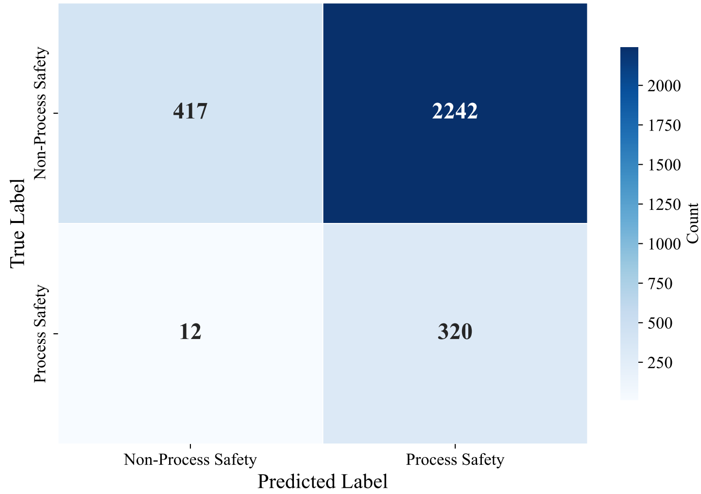
Confusion Matrix — GERMAN_MANUAL (snowflake-arctic-embed-l-v2.0, random_forest)
