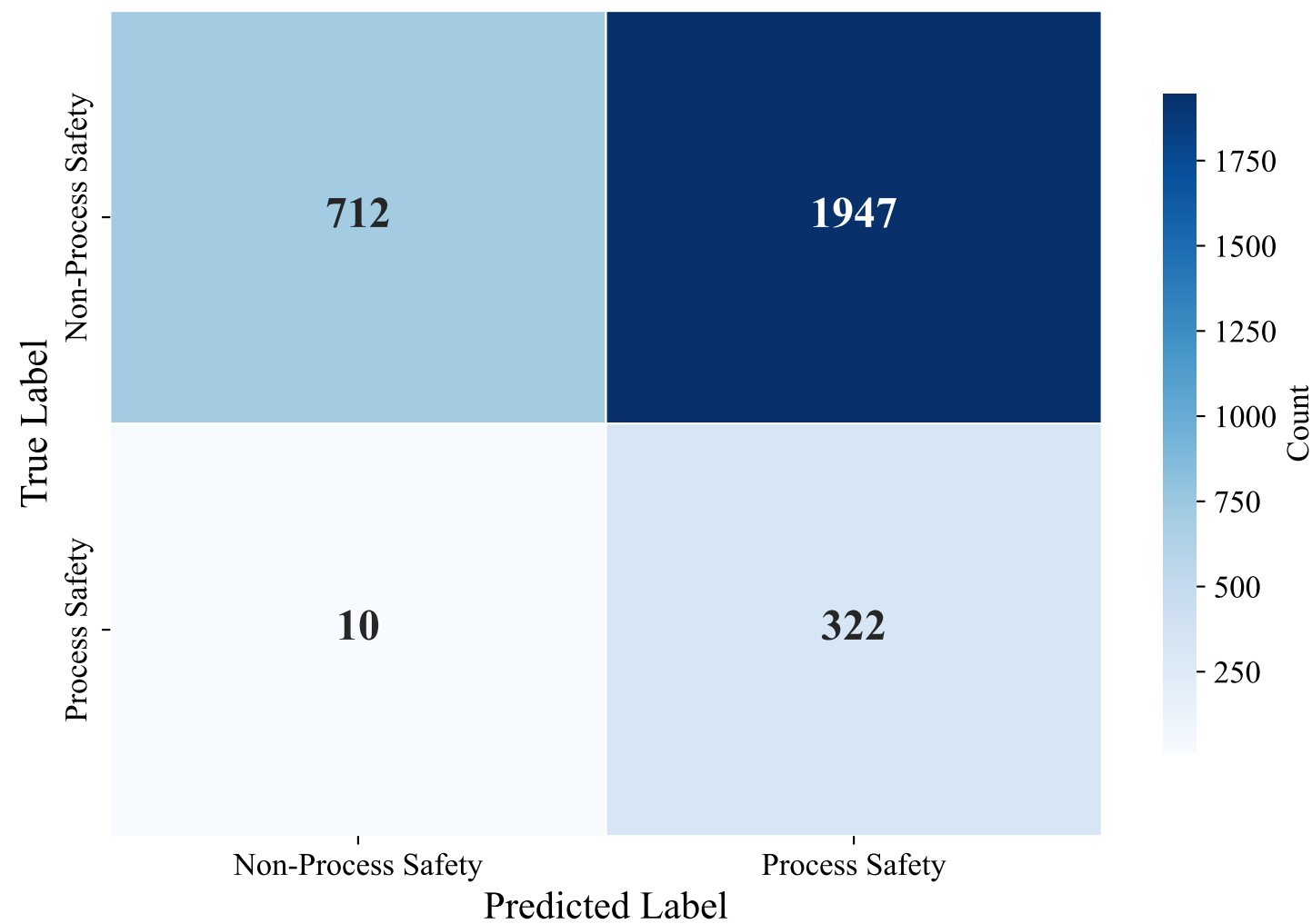
Confusion Matrix — GERMAN_MANUAL (snowflake-arctic-embed-l-v2.0, svm_linear)
