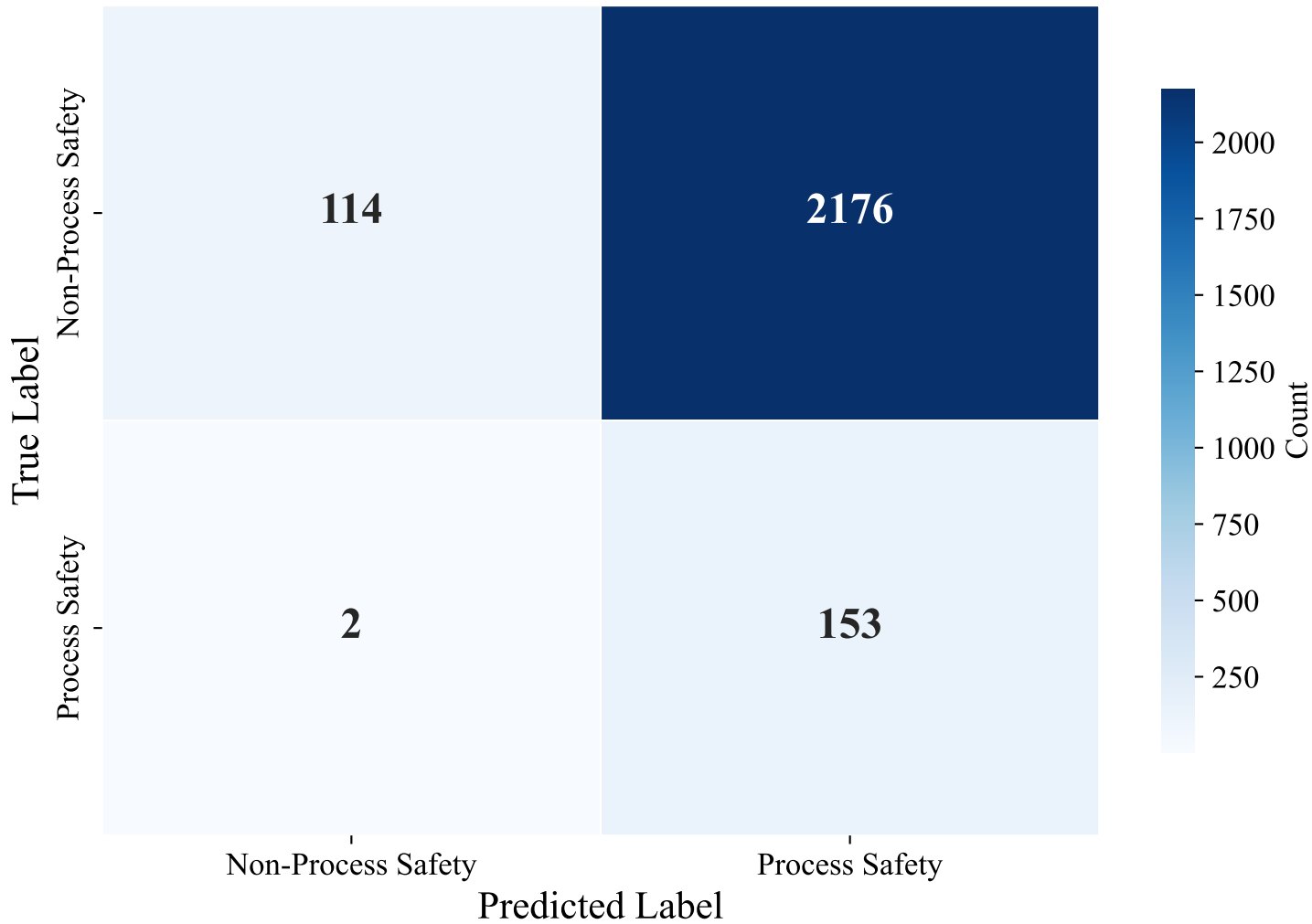
Confusion Matrix — SWEDISH_MANUAL (bert-base-multilingual-uncased, svm_linear)
