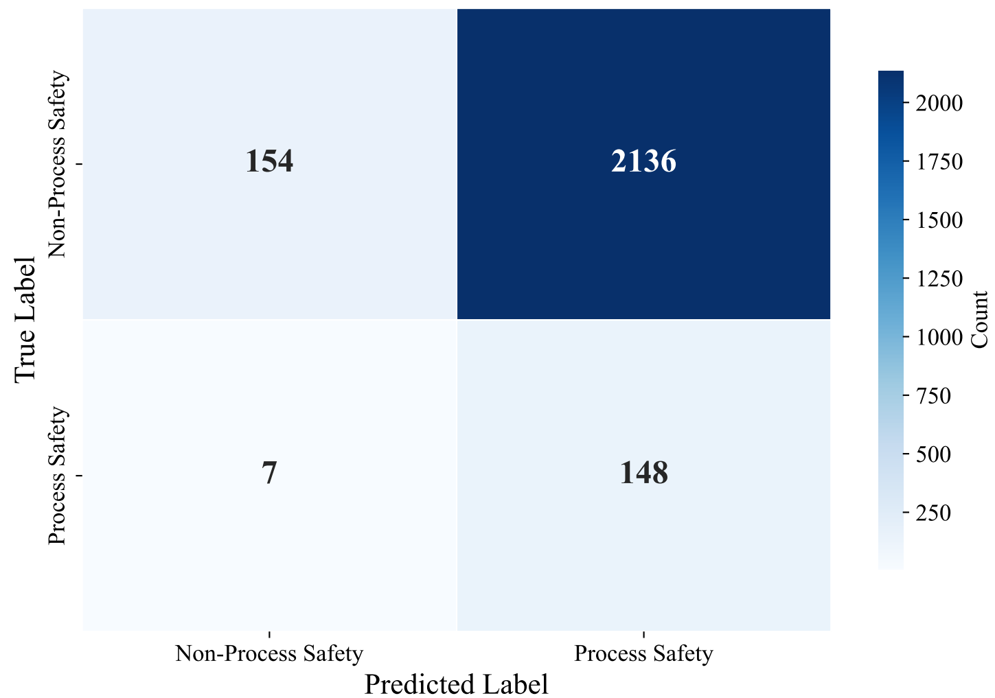
Confusion Matrix — SWEDISH_MANUAL (paraphrase-multilingual-mpnet-base-v2, lightgbm)
