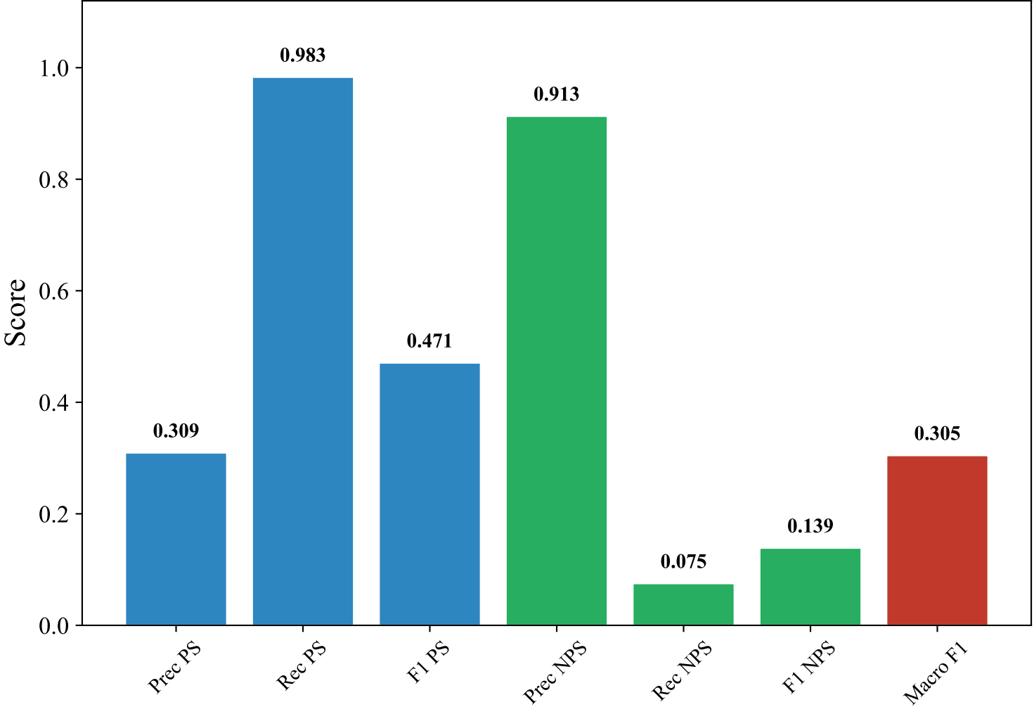
Classification Metrics — DUTCH_MANUAL (bert-base-multilingual-uncased, lightgbm)
