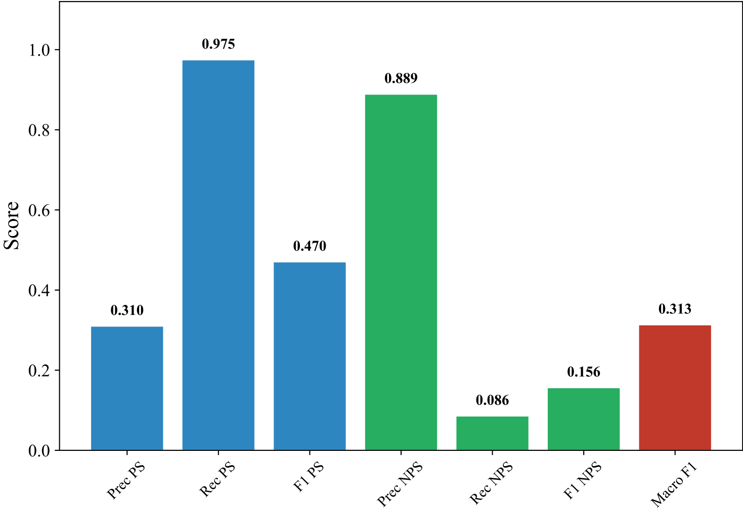
Classification Metrics — DUTCH_MANUAL (bert-base-multilingual-uncased, xgboost)
