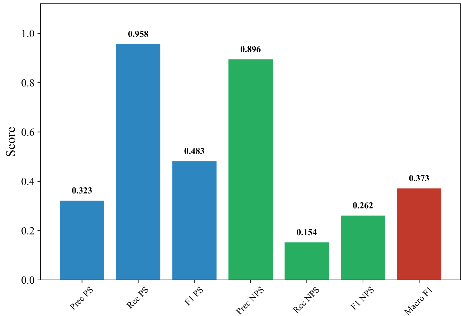
Classification Metrics — DUTCH_MANUAL (multilingual-e5-large-instruct, lightgbm)
