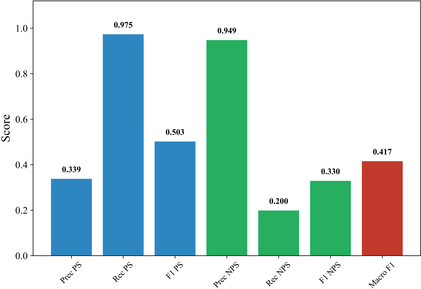
Classification Metrics — DUTCH_MANUAL (multilingual-e5-large-instruct, svm_rbf)
