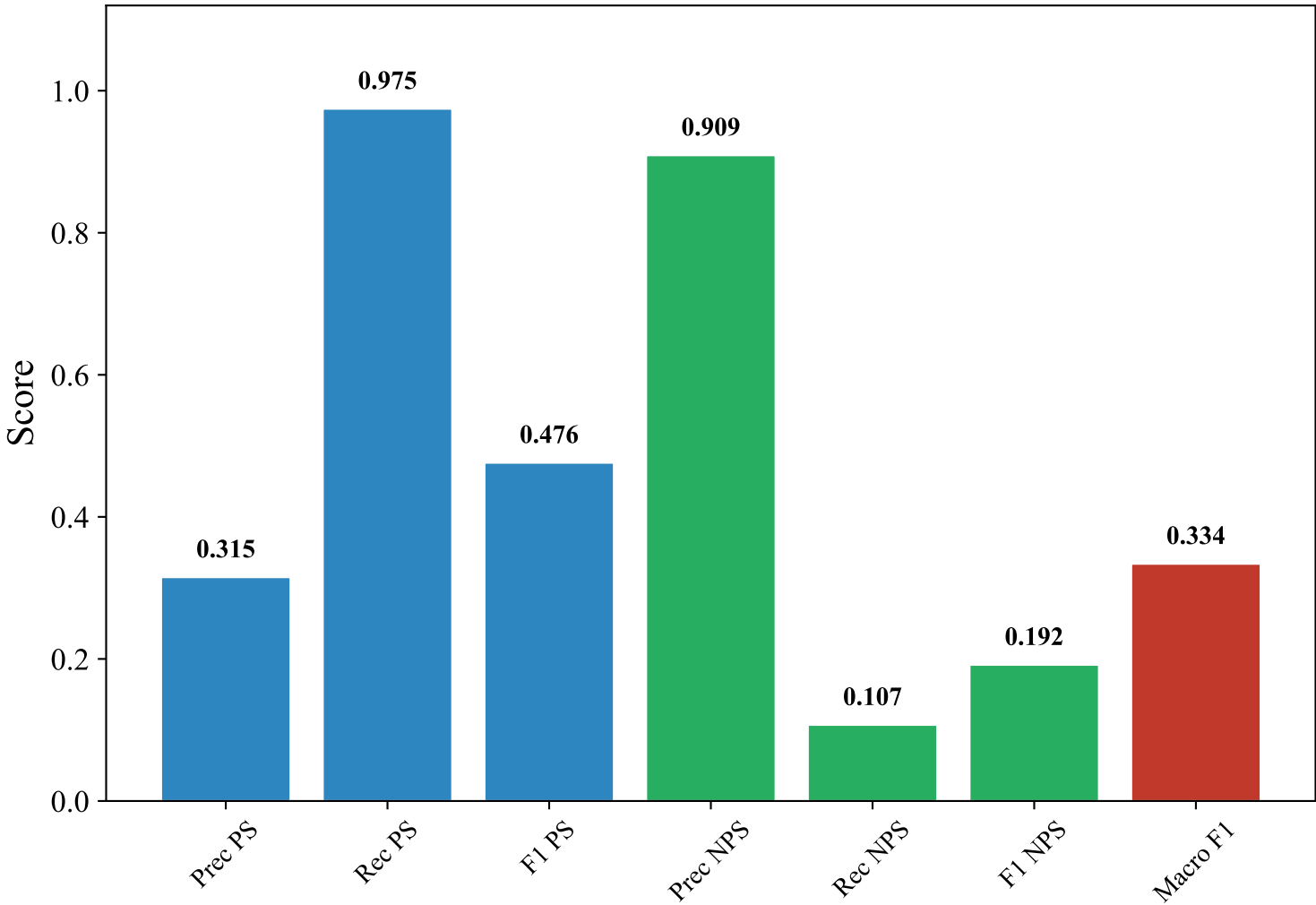
Classification Metrics — DUTCH_MANUAL (multilingual-e5-large-instruct, xgboost)
