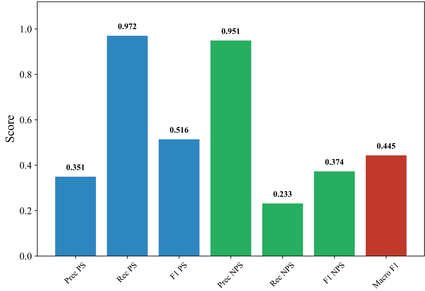
Classification Metrics — ENGLISH_MANUAL (bert-base-multilingual-uncased, svm_rbf)
