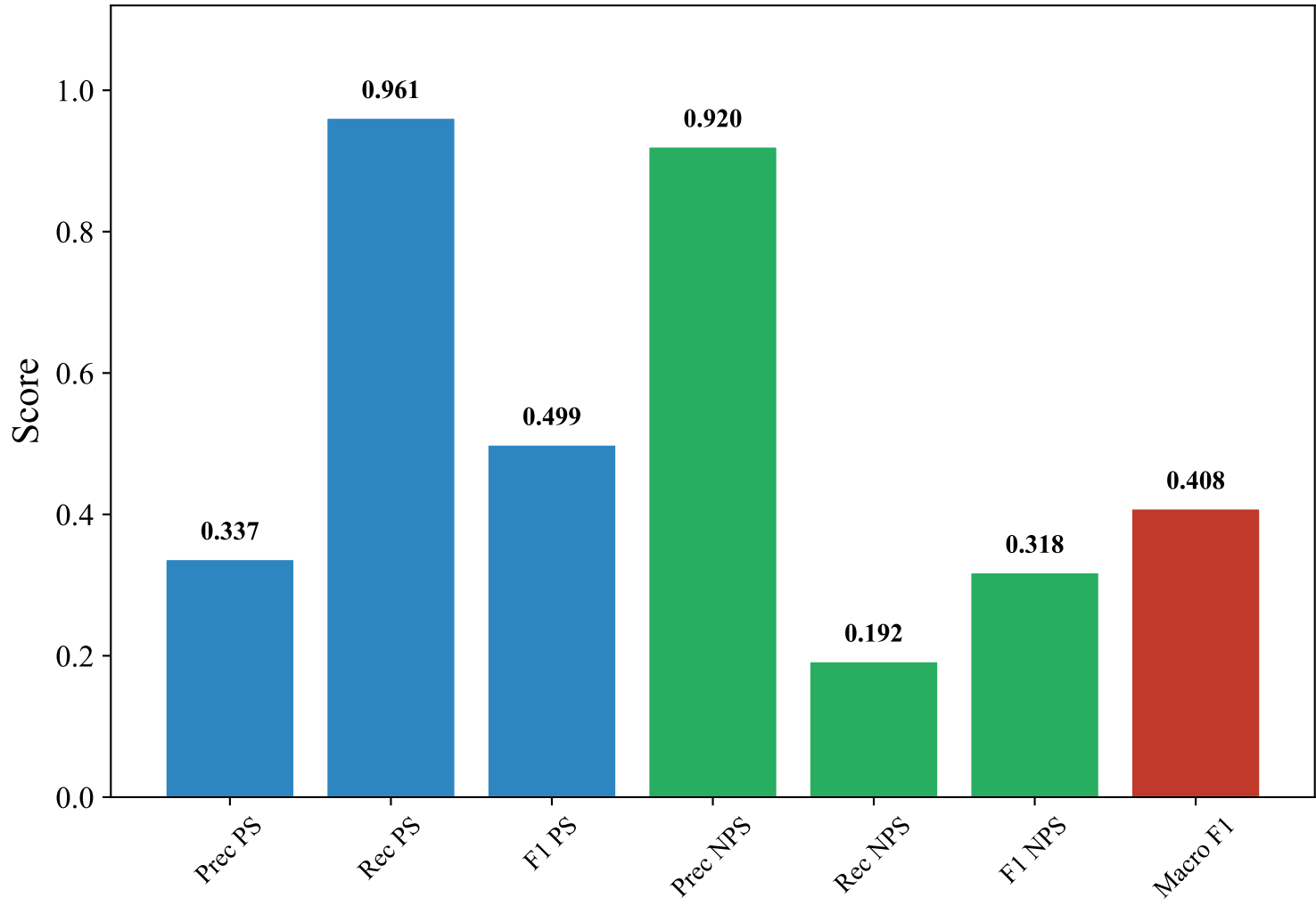
Classification Metrics — ENGLISH_MANUAL (bert-base-multilingual-uncased, xgboost)
