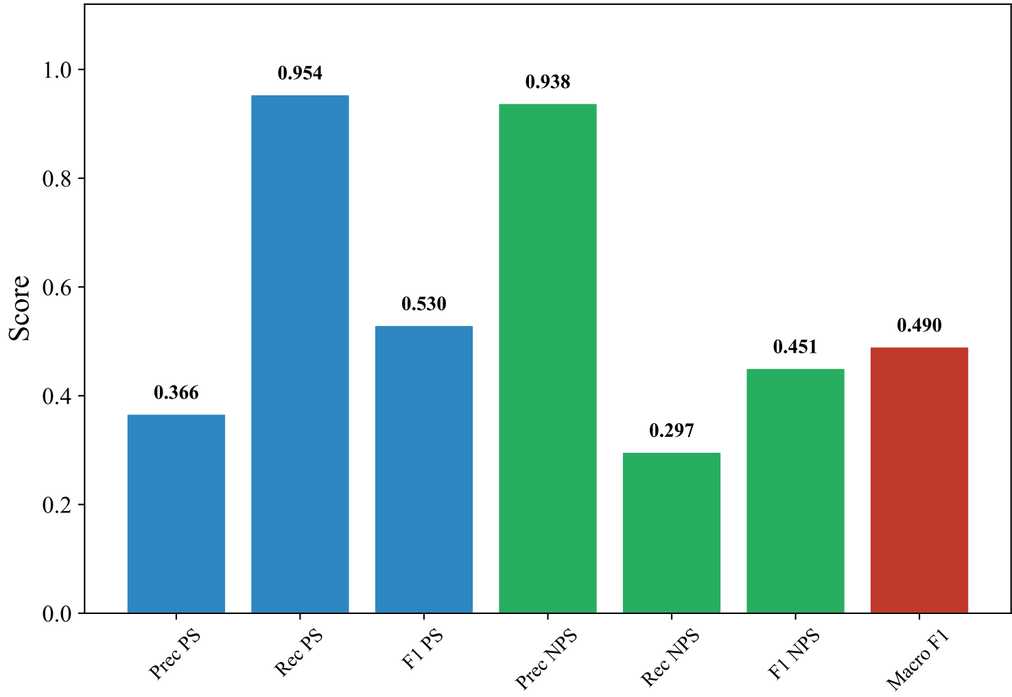
Classification Metrics — ENGLISH_MANUAL (paraphrase-multilingual-mpnet-base-v2, svm_linear)
