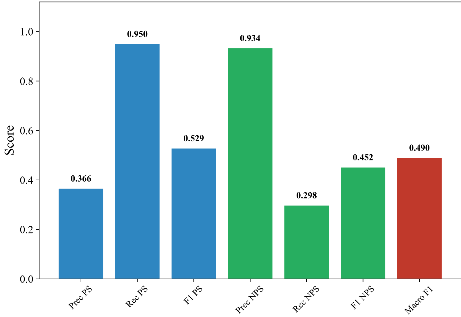
Classification Metrics — ENGLISH_MANUAL (snowflake-arctic-embed-l-v2.0, svm_linear)
