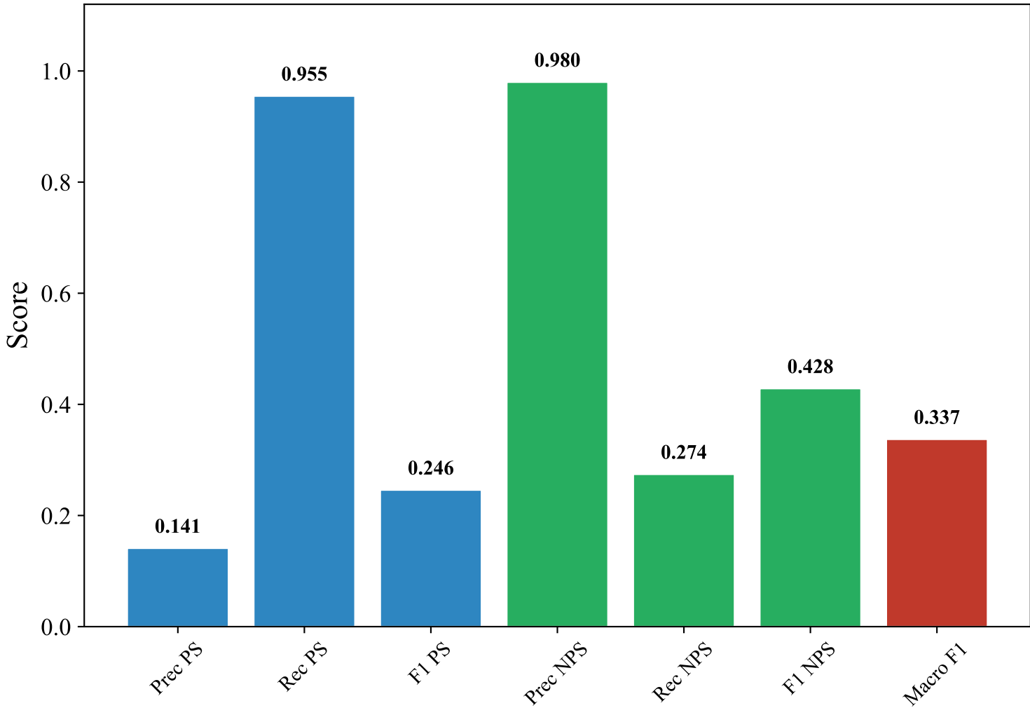
Classification Metrics — GERMAN_MANUAL (multilingual-e5-large-instruct, xgboost)
