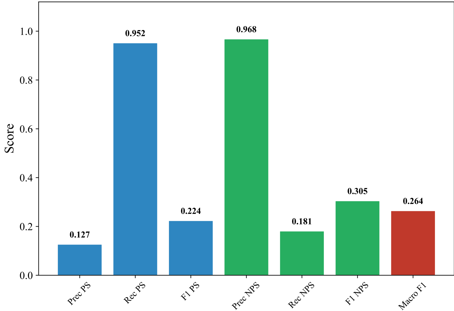
Classification Metrics — GERMAN_MANUAL (paraphrase-multilingual-MiniLM-L12-v2, svm_linear)
