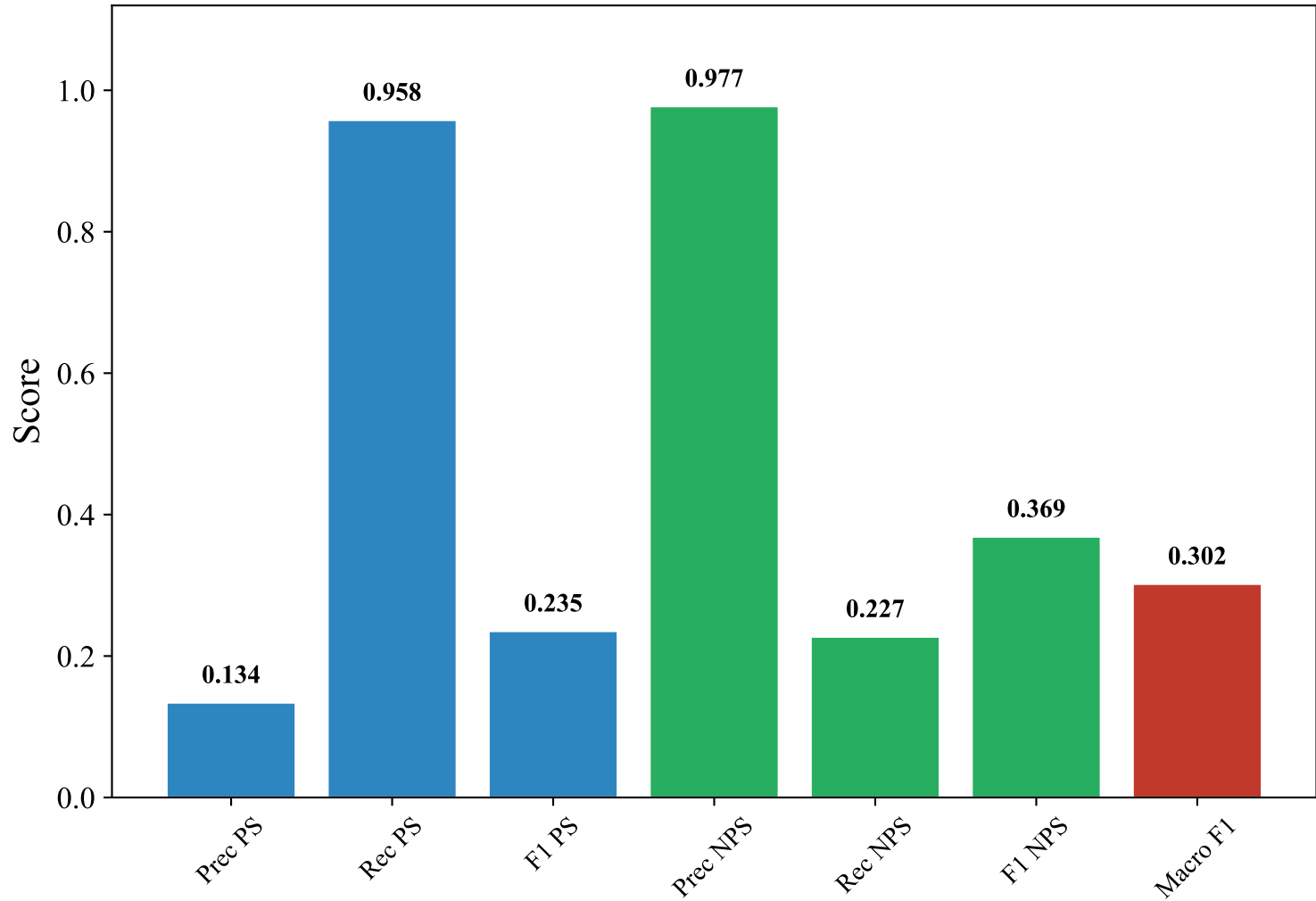
Classification Metrics — GERMAN_MANUAL (paraphrase-multilingual-MiniLM-L12-v2, svm_rbf)
