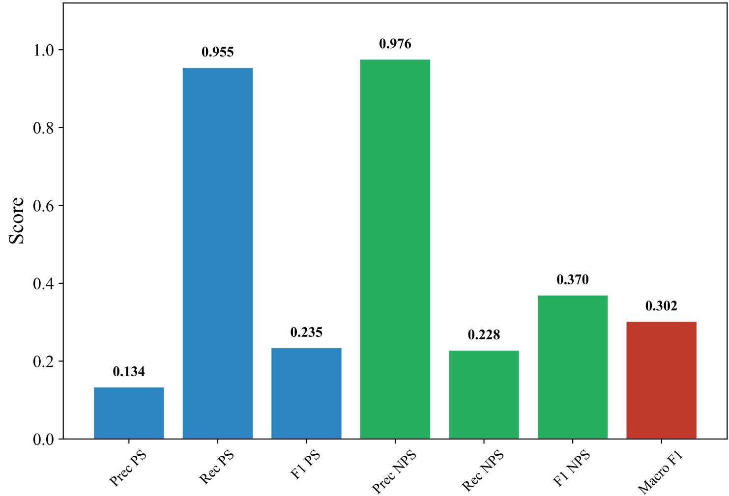
Classification Metrics — GERMAN_MANUAL (paraphrase-multilingual-mpnet-base-v2, xgboost)
