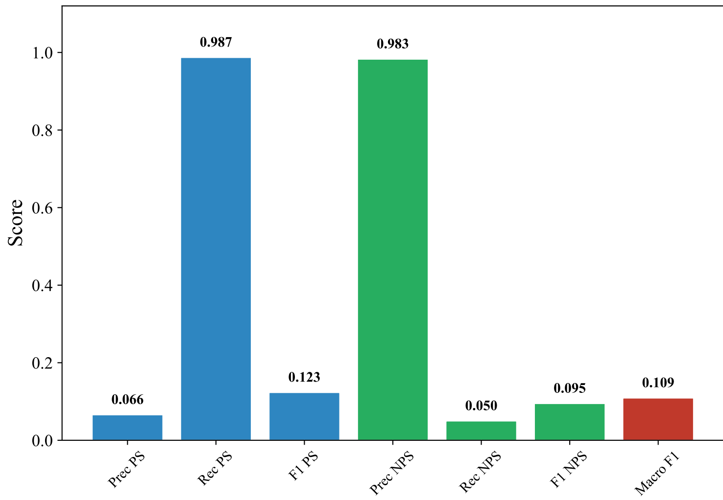
Classification Metrics — SWEDISH_MANUAL (bert-base-multilingual-uncased, svm_linear)
