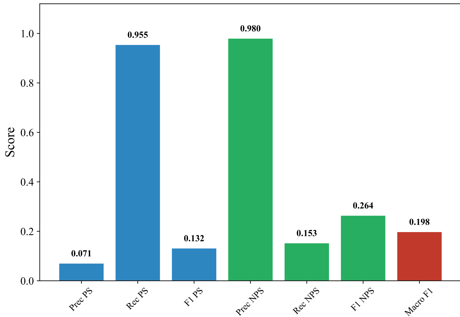
Classification Metrics — SWEDISH_MANUAL (paraphrase-multilingual-MiniLM-L12-v2, svm_linear)
