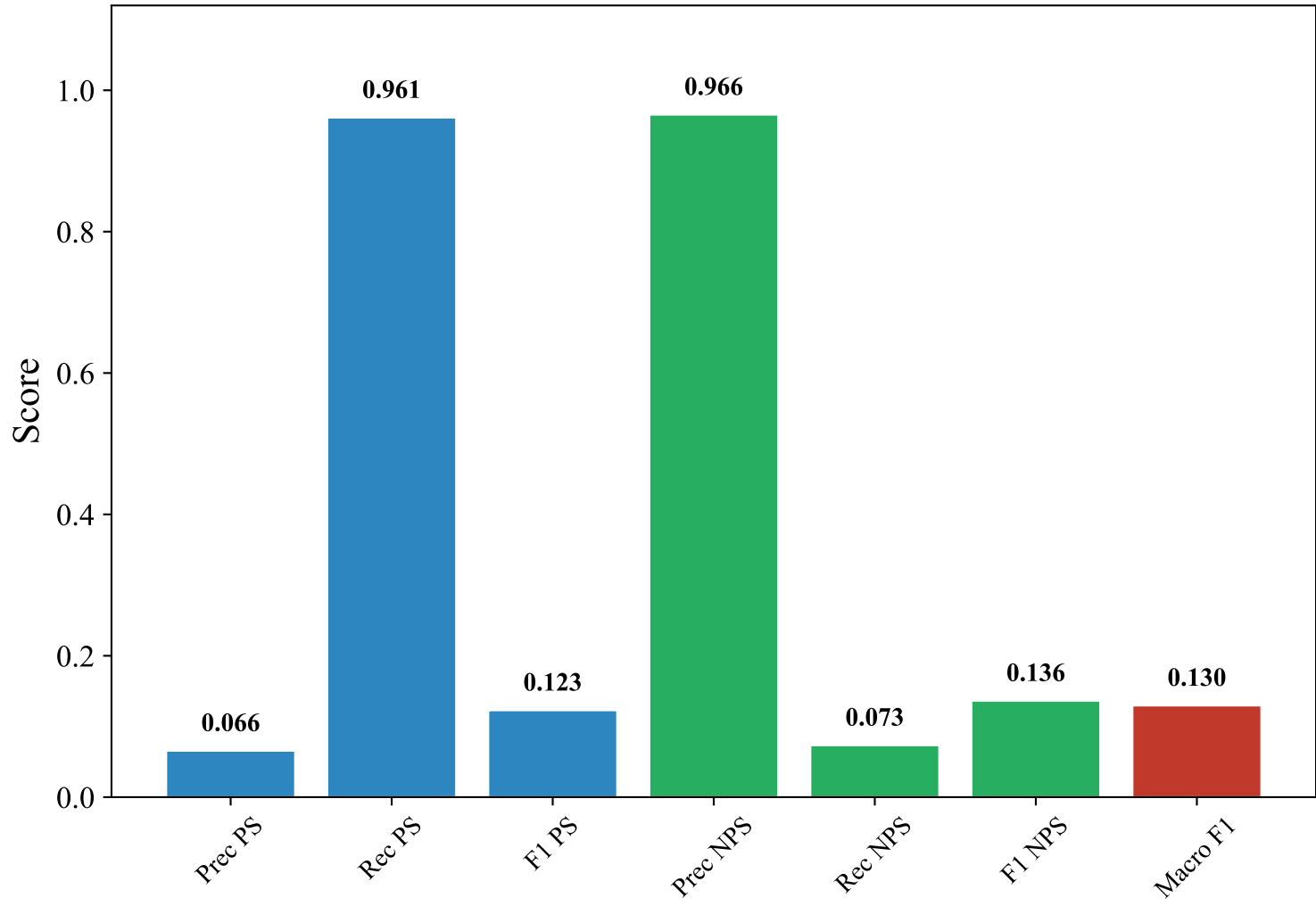
Classification Metrics — SWEDISH_MANUAL (paraphrase-multilingual-mpnet-base-v2, svm_rbf)
