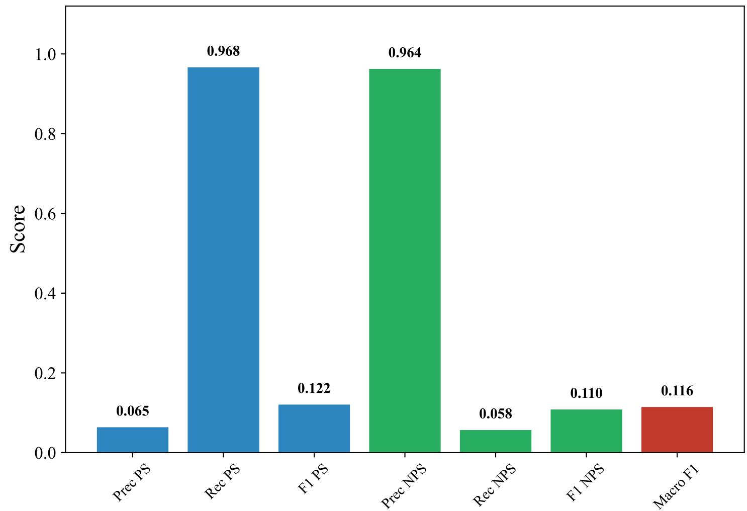
Classification Metrics — SWEDISH_MANUAL (paraphrase-multilingual-mpnet-base-v2, xgboost)
