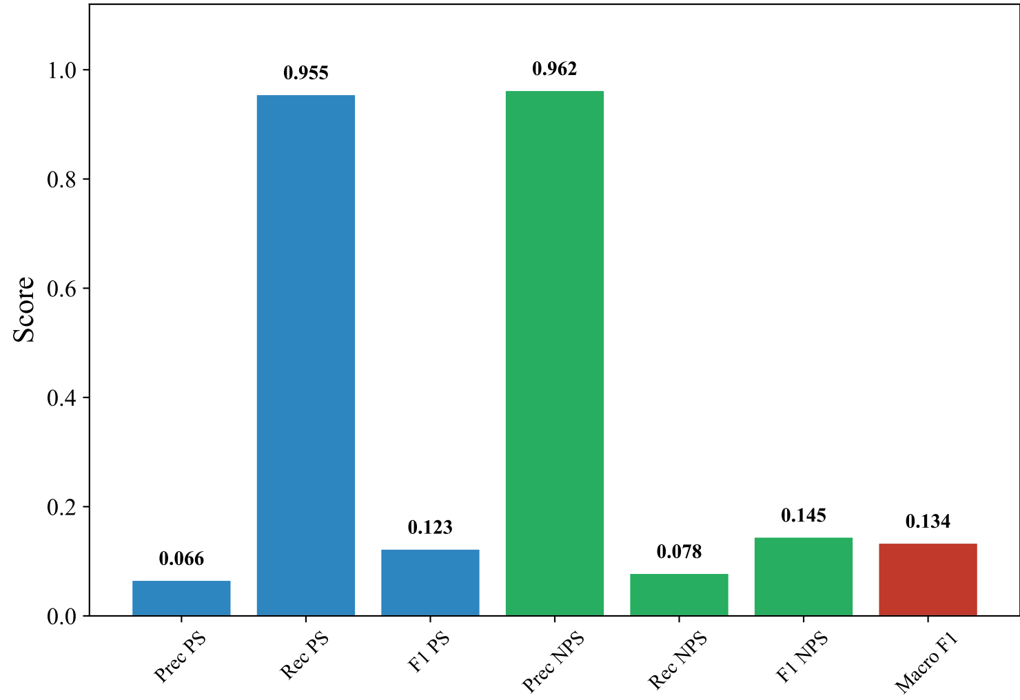
Classification Metrics — SWEDISH_MANUAL (snowflake-arctic-embed-l-v2.0, lightgbm)
