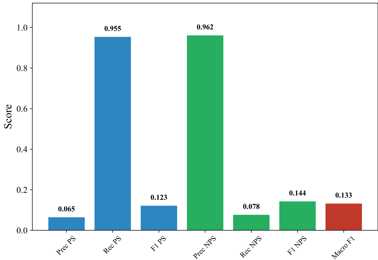
Classification Metrics — SWEDISH_MANUAL (snowflake-arctic-embed-l-v2.0, xgboost)
