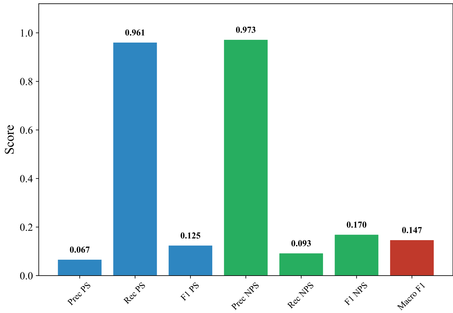
Classification Metrics — SWEDISH_MANUAL (xlm-roberta-base, svm_linear)
