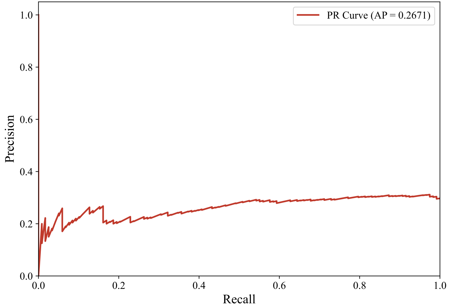
Precision-Recall Curve — DUTCH_MANUAL (bert-base-multilingual-uncased, xgboost)
