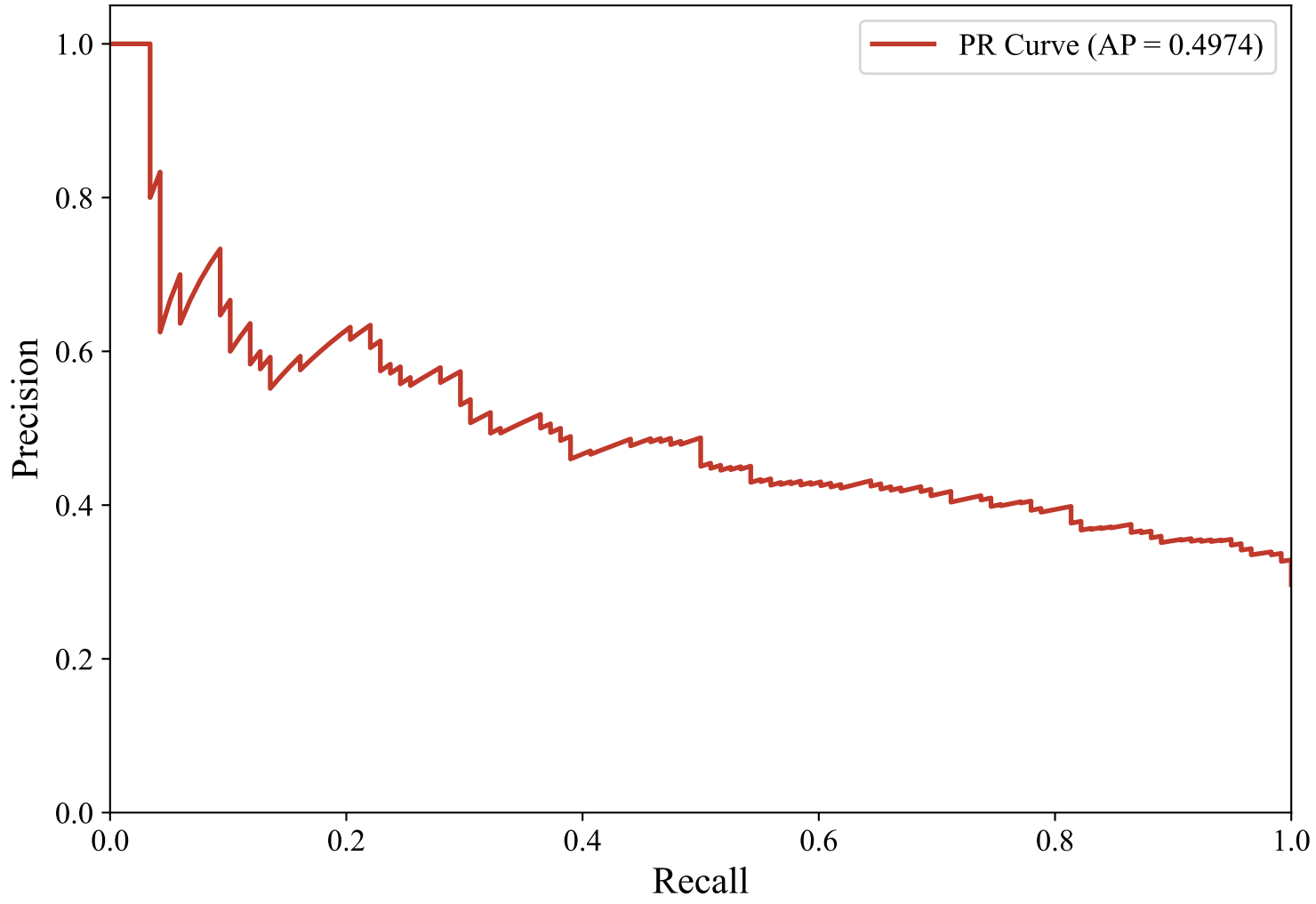
Precision-Recall Curve — DUTCH_MANUAL (multilingual-e5-large-instruct, svm_linear)
